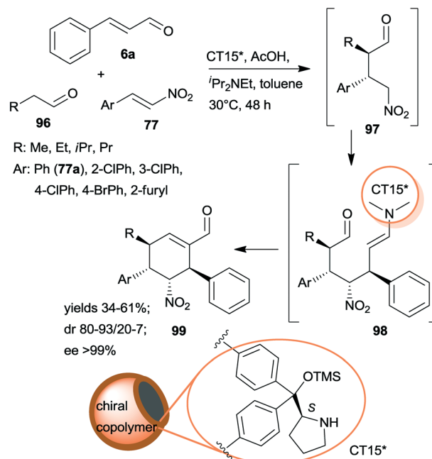
Scheme 29 Tricomponent asymmetric triple cascade reaction catalysed by multi-hollow copolymer microparticles containing immobilized CA6*; AC: aldol condensation. 163
