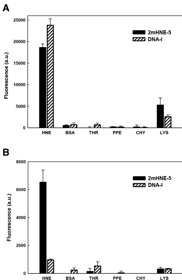
Fig. 2 Specificity of binding of 2mHNE-5 and DNA-I to different proteins in the presence of 150 mM NaCl (A) or 500 mM NaCl, 66 µg mL -1 yeast tRNA (B). BSA, bovine serum albumin; THR, thrombin; PPE, porcine pancreas elastase; CHY, chymotrypsin; LYS, lysozyme. Data are the average and s.d. of three independent determinations.
