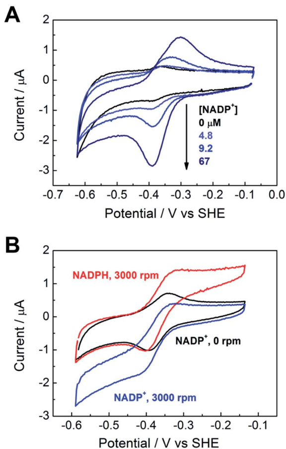
Fig. 3 Cyclic voltammetry of \text{NADP}^+/\text{NADPH} . (A) Diffusion-controlled, quasi-reversible interconversion of \text{NADP}^+ and \text{NADPH} at a stationary FNR@ITO/PGE electrode, with increasing amounts of \text{NADP}^+ , scan rate 5 \text{ mV s}^{-1} . (B) Effect of electrode rotation at scan rate 1 \text{ mV s}^{-1} : stationary electrode with 50 \text{ } \mu\text{M} \text{NADP}^+ (black) and under 3000 rpm rotation with 50 \text{ } \mu\text{M} \text{NADP}^+ (blue) or 50 \text{ } \mu\text{M} \text{NADPH} (red). Other conditions: buffer solution containing 25 \text{ mM} MES, 25 \text{ mM} TAPS, pH 8.0, 20 \text{ } ^\circ\text{C} , purged with Ar before measurement.
