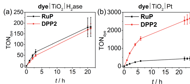
Fig. 4 (a) Photocatalytic activity of \text{DPP2}|\text{TiO}_2|\text{H}_2\text{ase} and \text{RuP}|\text{TiO}_2|\text{H}_2\text{ase} . Conditions: 2.5 mg \text{TiO}_2 , 50 pmol [ \text{NiFeSe} ]- \text{H}_2\text{ase} , 0.05 \mu\text{mol} of DPP2 or RuP , in 3 mL AA-MES solution (0.1 M, pH 6); (b) photocatalytic activity of \text{DPP2}|\text{TiO}_2|\text{Pt} and \text{RuP}|\text{TiO}_2|\text{Pt} . Conditions: 2.5 mg pre-platinised \text{TiO}_2 , 0.05 \mu\text{mol} of DPP2 or RuP , in 3 mL AA solution (0.1 M, pH 4.5). In both cases the samples were irradiated with UV-filtered solar light (100 \text{mW cm}^{-2} , AM 1.5G, \lambda > 420 nm) at 25 °C.
