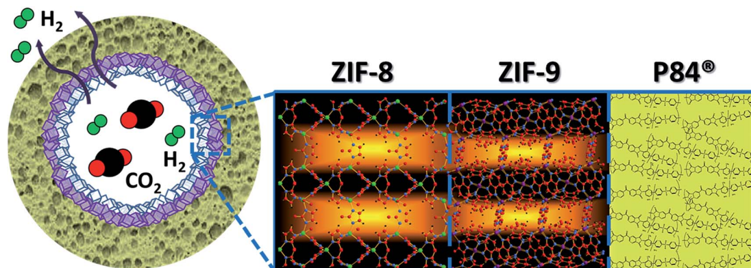
Fig. 1 Scheme of the double-layered ZIF-8/ZIF-9 membrane inside a polymeric (P84) hollow fiber for H 2 /CO 2 separation.
