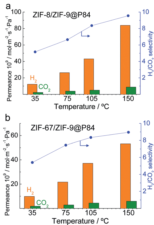
Fig. 6 Double-layered ZIF-8/ZIF-9 (a) and ZIF-67/ZIF-9 (b) membrane permeation properties in the H_2/CO_2 mixture separation as a function of temperature.
