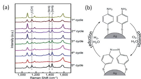
Fig. 4 SERS spectra (a) and schematic illustration (b) of the reversible reactions of PATP to DMAB. 36
