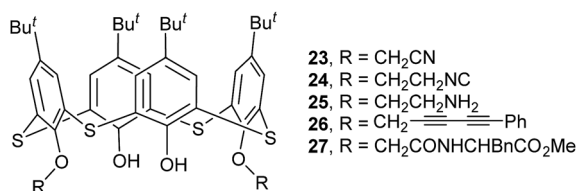
Fig. 18 Structures of compounds 23–27.
