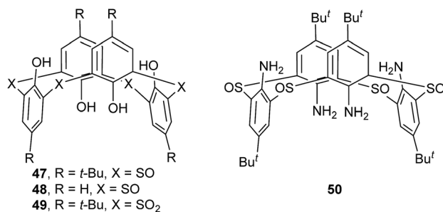
Fig. 39 Structures of compounds 47 – 50 .
