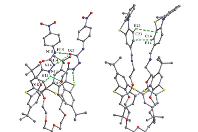
Fig. 70 Crystal structures of 74 (left) showing H-bonds, and 75 (right) showing C–H \cdots\pi contacts.
