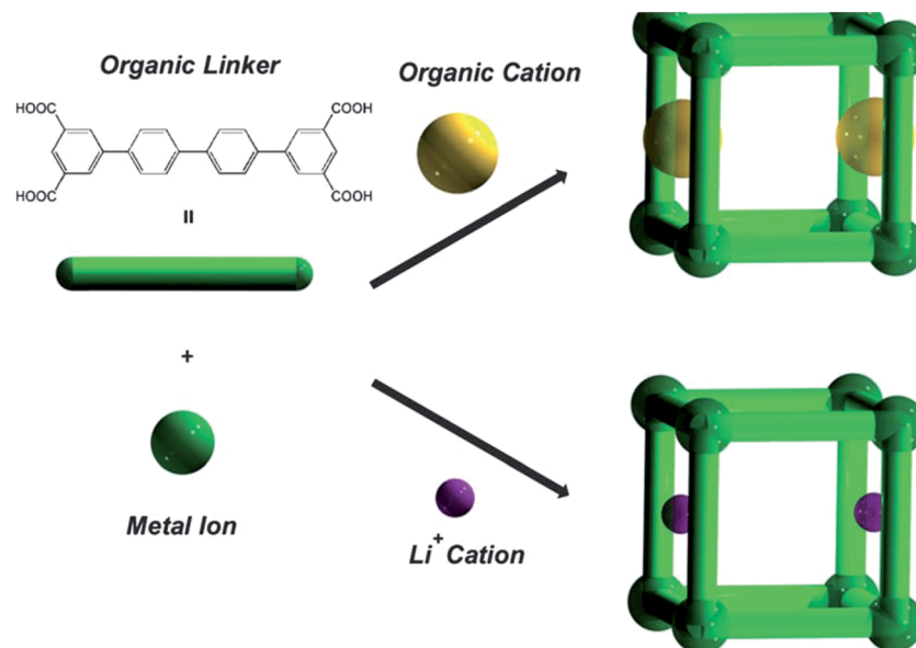
Fig. 14 A schematic representation of the construction of modulated MOFs in \{[In(L^7)] \cdot \text{solv}\}_\infty (69) with different pore gates. Reproduced with permission from ref. 109, copyright 2011, Royal Society of Chemistry.
