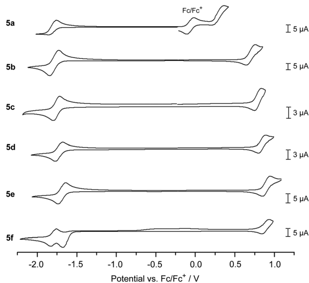
Fig. 3 Cyclic voltammograms of 5a–f (1 mm* in CH 2 Cl 2 , 0.1 m n -Bu 4 NPF 6 , scan rate 0.1 V s -1 (for 5c 0.2 V s -1 ), 5c , 5d , and 5e with a Pt-electrode, 5b , 5a , and 5f with a GC-electrode). † *Due to solubility issues the concentration of 5a was lower.
