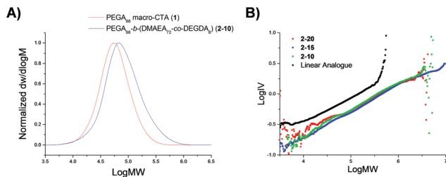
Fig. 1 (a) RI traces of the linear PEGA 98 macro CTA (1, red) and PEGA 98 - b -(DMAEA 72 - co -DEGDA 8 ) (2-10, blue) obtained by SEC analysis. (b) Triple detection SEC Mark-Houwink curves for PEGA 98 armed particles with varying crosslinking densities compared to the linear analogue PEGA 98 - b -(DMAEA 60 - co -MA 13 ), in DMF with 5 mM NH 4 BF 4 and PMMA as standards.
