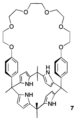
Fig. 2 Strapped calix[4]pyrrole 7 .
