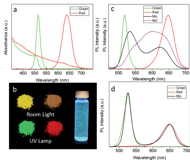
Fig. 2 (a) UV-visible absorption and PL spectra of green-emitting CsPbBr 3 and red-emitting CsPb(Br/I) 3 POSS-coated NCs. (b) Photographs of CsPbBr 3 and CsPb(Br/I) 3 POSS coated NC powders under room light and UV light, and a vial with a CsPbBr 3 POSS-NC suspension in water after 10 weeks storage, under UV light. (c) Solid state PL spectra of non-capped CsPbBr 3 (sample Green) and CsPb(Br/I) 3 (sample Red) NC powders, and of their 1 : 1 molar% mixture taken immediately after mixing (sample Mix) and after 5 min of the solid state reaction (sample Mix'). (d) Solid state PL of POSS-capped CsPbBr 3 (sample Green) and CsPb(Br/I) 3 (sample Red) POSS-NC powder NCs, and of their 1 : 1 molar% mixture.
