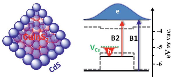
Scheme 1 (Left) schematic structure and (right) quasi-type II band alignment in \text{CuInS}_2/\text{CdS} core/shell QDs. Bulk band edges of \text{CuInS}_2 and CdS (gray dashed lines), electron and hole energy levels in the core and shell (black solid lines), hole trapping levels associated with Cu vacancy ( V_{\text{Cu}} , green dashed line), lowest energy transitions in the CdS (B1) and \text{CuInS}_2 (B2). In the lowest excited state, electron and hole wavefunctions are delocalized among core and shell and localized in the core ( V_{\text{Cu}} ), respectively.
