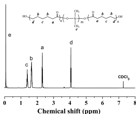
Fig. 2 1 H NMR spectrum of the PCL- b -PDMS- b -PCL triblock copolymer.
