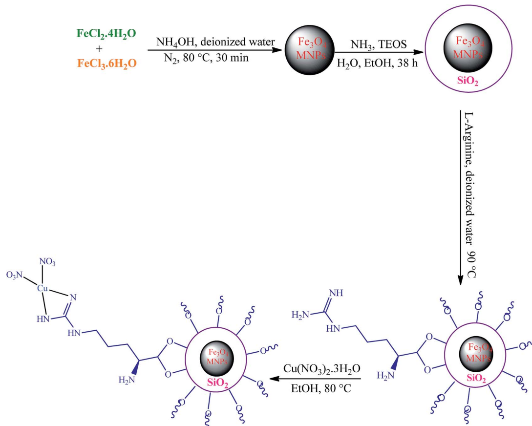
Scheme 1 General route for the synthesis of Cu(II) immobilized on \text{Fe}_3\text{O}_4@SiO_2@L -arginine.
