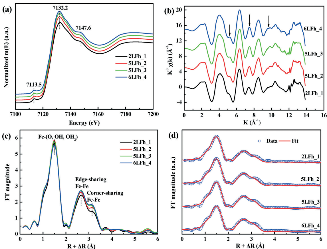
Fig. 3 Fe K-edge XANES (a); the k^3 -weighted EXAFS spectra, where the arrows indicate the main oscillations affected by the crystallite size (b); the Fourier transforms (magnitude) of the k^3 -weighted EXAFS spectra (c); the radial distribution functions (symbols) and their fits using the Michel model (red curves) (d).
