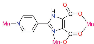
Fig. 13 Section of the structure of [\text{Mn}_2(\text{Hpidc})(\text{H}_2\text{O})\cdot 2\text{H}_2\text{O}]_n . 78
