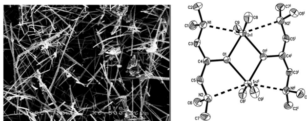
Fig. 23 Left, SEM image of \text{In}_2\text{O}_3 deposited from the reaction of \text{InMe}_3 and \text{HOCH}_2\text{CH}_2\text{OMe} at 550 \text{ }^\circ\text{C} , and right, X-ray structure of [\text{Me}_2\text{In}(\text{OCH}(\text{CH}_2\text{NMe}_2)_2)]_2 with thermal ellipsoids shown at the 50% probability level. Reproduced with permission from ref. 171. Copyright 2012 American Chemical Society.
