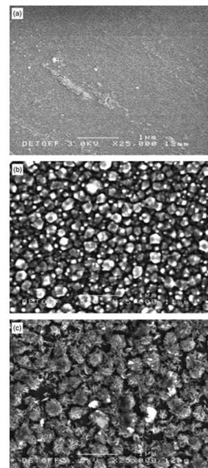
Fig. 24 SEM of films grown from AACVD deposition of \text{InMe}_3 and \text{MeOH} at (a) 400 \text{ }^\circ\text{C} ; (b) 450 \text{ }^\circ\text{C} ; and (c) 500 \text{ }^\circ\text{C} . Reproduced with permission from ref. 176 Copyright 2013 Royal Australian Chemical Institute.
