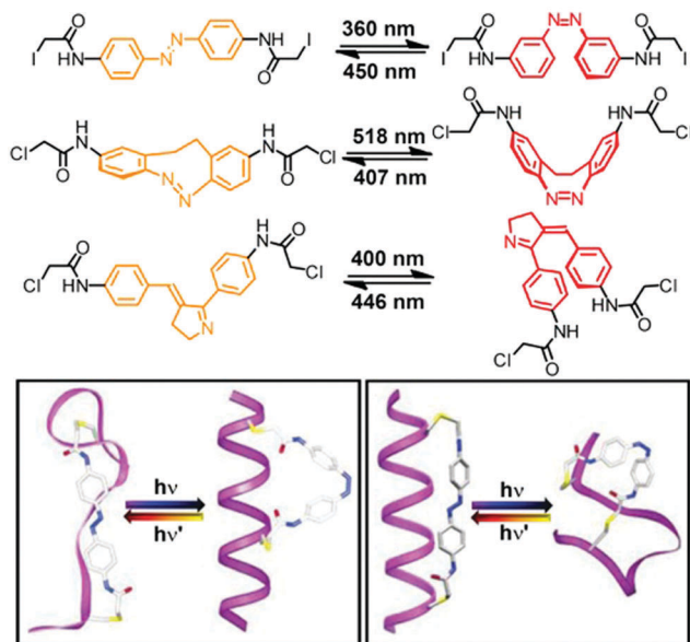
Fig. 7 Photoswitches that have been used as tethers to covalently link two side chain residues in peptide based foldamers in the loop approach (top). Turn-on (bottom left) and turn-off (bottom right) helices with the E - and Z -configured tethers connecting the i and i + 7 positions and the i and i + 11 positions of the peptide \alpha -helix, respectively. 80
