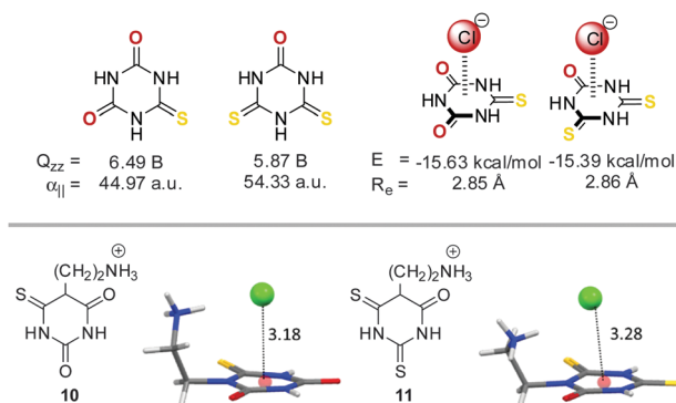
Fig. 6 Molecular structures, quadrupole moments and molecular polarizabilities of selected thio cyanuric acid derivatives and their corresponding anion- \pi complexes with chloride (including the calculated interaction energies and equilibrium distances). Additionally, the ion pairs of the ethylene ammonium-substituted chloride salts of the thio- ( 10 ) and dithiocyanuric acids ( 11 ) are shown as observed in the solid state. 19c
