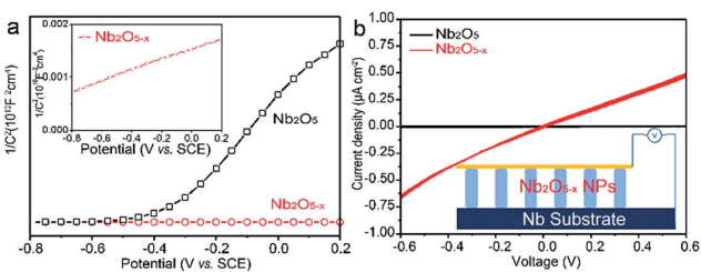
Fig. 3 (a) Mott-Schott plots of \text{Nb}_2\text{O}_5 and \text{Nb}_2\text{O}_{5-x} NPs films at a frequency of 1 kHz in the dark; (b) comparison of I - V curves of the samples; the inset is the schematic of the measurement.
