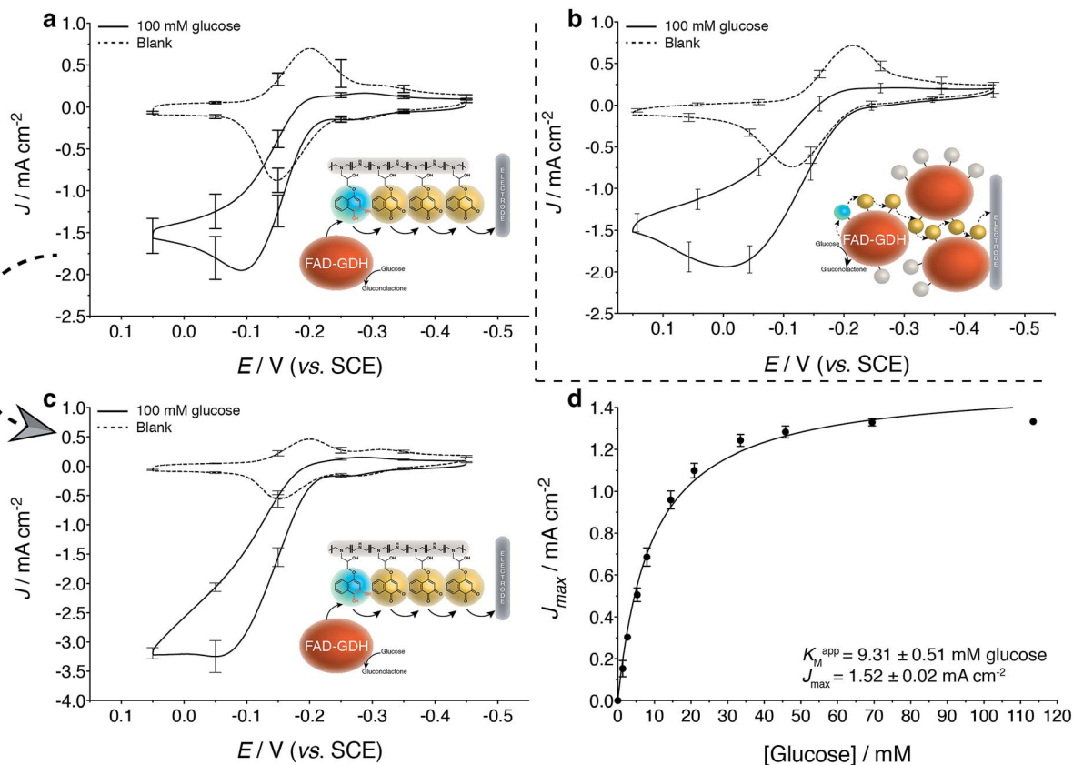
Fig. 3 Electrochemical evaluation of carbon electrodes modified with a NQ redox hydrogel (NQ-4-LPEI) and NQ-labeled GDH (NQ-4-GDH). (a) Cyclic voltammogram of NQ-4-LPEI GDH bioelectrodes in the absence and presence of glucose. (b) Cyclic voltammogram of NQ-4-GDH bioelectrodes in the absence and presence of glucose. NQ-4-GDH was covalently immobilized with hydrophobically modified linear polyethyleneimine ( \text{C}_8\text{LPEI} ). (c) NQ-4-LPEI GDH redox hydrogels were scaled to simple carbon paper electrodes (Toray) to demonstrate performance on an applicable and disposable electrode. (d) Apparent Michaelis–Menten kinetics of the resulting NQ-4-LPEI GDH bioelectrode (from c). All electrodes were evaluated at pH 6.5 (citrate/phosphate buffer, 0.2 M). Cyclic voltammograms were performed at 10 \text{ mV s}^{-1} and amperometric i-t experiments were performed at 0 V (vs. SCE). Error bars report one standard deviation ( n = 3 ). Electrodes were modified with carbon nanotubes prior to functionalization.
