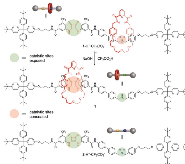
Fig. 2 Acid–base control of the position of the macrocycle in rotaxane 1 (iminium catalysis 'on'; hydrogen bond catalysis 'off')/ 1 \cdot H^+ \cdot CF_3CO_2^- (iminium catalysis 'off'; hydrogen bond catalysis 'on') and the structure of the corresponding thread 2 ( H^+ \cdot CF_3CO_2^- (both iminium catalysis and hydrogen bond catalysis 'on')).
