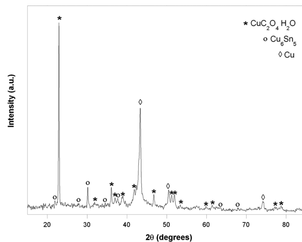
Fig. 4 WA-XRD spectrum and peaks assignment for \text{Cu}(\text{C}_2\text{O}_4) \cdot \text{H}_2\text{O} precipitate obtained from the leaching of 10 g of test specimen by citric acid 3M at room temperature and \text{H}_2\text{O}_2 35% addition.
