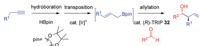
Scheme 25 Allylboration with Ir(i)-complex/TRIP relay system.
