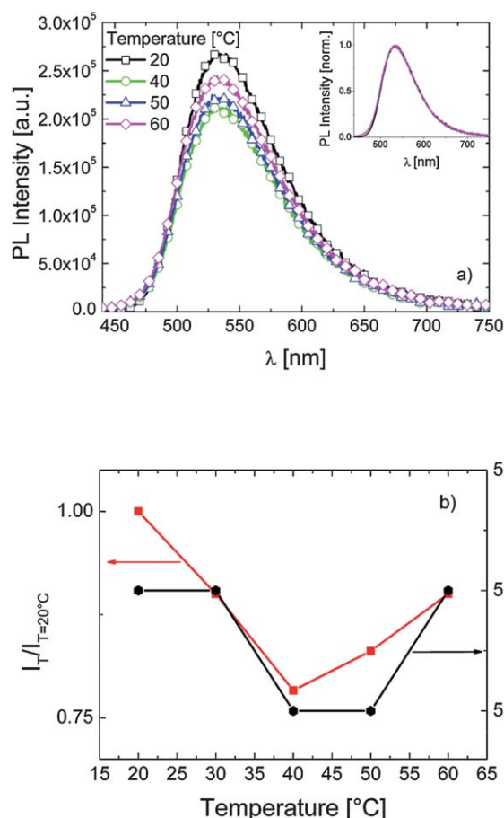
Fig. 4 (a) The fluorescence spectra of P-3 in PBS ( 0.1 \text{ g L}^{-1} ) at various temperatures. Excitation was at 430 nm. The inset depicts the emission spectra at 20 and 60 °C normalized to their maximum emission intensity. (b) The correlation between \lambda_{\text{PL,max}}^{\text{PL}} , the relative emission intensity ( I_T/I_{T=20^\circ\text{C}} ), and the temperature of the solution. Data are taken from the spectra in (a).
