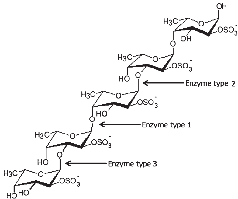
Fig. 1 Enzymatic attack patterns of \alpha -L-fucoidan endohydrolase and fucosidase, respectively: For simplicity, we have distinguished the cleavage patterns as type 1 for (1 \rightarrow 3)- \alpha -L-fucoidan endohydrolase and type 2 for (1 \rightarrow 3)- \alpha -L-fucoidan endohydrolase; and the exo -action, EC 3.2.1.51, as type 3. (Since the EC 3.2.1.44 fucoidanase activity only designates catalysis of the endo -hydrolysis of (1 \rightarrow 2)- \alpha -L-fucosides, the enzymes type 1 and type 2 \alpha -L-fucoidan endohydrolases are in principle not EC categorized.) References in Table 4.
