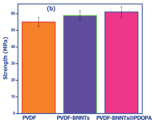
Fig. 9 Comparative tensile tests performed on PVDF, PVDF/BNNTs, PVDF/BNNT@PDOPA composites: (a) elastic modulus and (b) yield strength.
