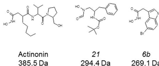
Fig. 1 Chemical structures of the PDF1B ligands used in the present study.
