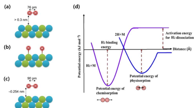
Fig. 1 (a) Physisorption, (b) chemisorption, (c) weakly bonded hydrogen, 29 (reproduced from ref. 29 with permission from Wiley, copyright 2015), and (d) one-dimensional potential energy profiles for physisorption and chemisorption processes plotted as a function of the separation distance between H 2 molecules and the substrate. Reprinted with permission, 25 (reproduced from ref. 25 with permission from Wiley, copyright 2025).
