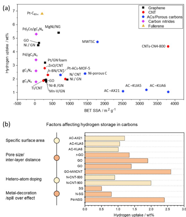
Fig. 7 (a) Comparison of the \text{H}_2 storage capacities of carbon-based adsorbents with respect to their specific surface area and (b) factors affecting the hydrogen storage in carbon-based materials.
