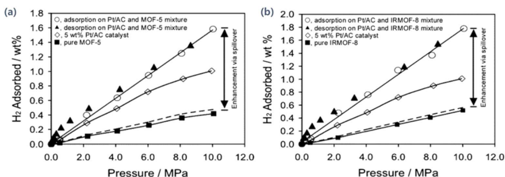
Fig. 10 Comparison of \text{H}_2 storage isotherms showing enhancement via the spillover effect for (a) pure MOF-5 and modified with Pt/Ac and (b) IRMOF-8 modified with Pt/Ac at 298 K 150 (reproduced from ref. 150 with permission from The American Chemical Society, copyright 2006).
