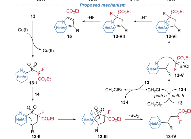
Scheme 6 Assembly of heteroarenes via the docking–migration–cyclization cascade.
