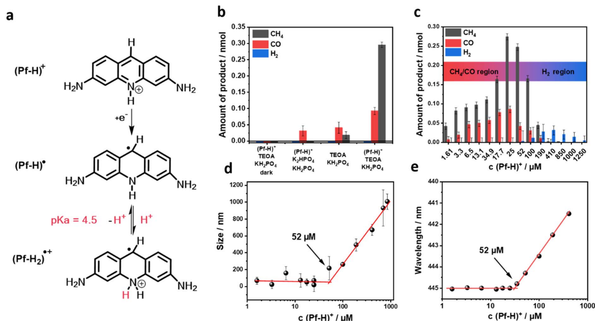
Fig. 1 (a) Relevant structures. (b) Rate of CH 4 , CO, and H 2 evolution at pH 7 after 1 h upon 1 sun irradiation with a Xe-lamp equipped with 1.5 AM filter. (c) Rate of CH 4 , CO, and H 2 evolution measured in aqueous solution of 4.28 vol% TEOA, 0.55 M KH 2 PO 4 , at pH 7, and with different concentrations of (Pf-H) + over 1 hour of irradiation. (d) DLS analysis in aqueous solution of 4.28 vol% TEOA, 0.55 M KH 2 PO 4 , at pH 7, and with different concentrations of (Pf-H) + . (e) Concentration-dependent shift in absorbance of aqueous solutions with 4.28 vol% TEOA, 0.55 M KH 2 PO 4 , and at pH 7.
