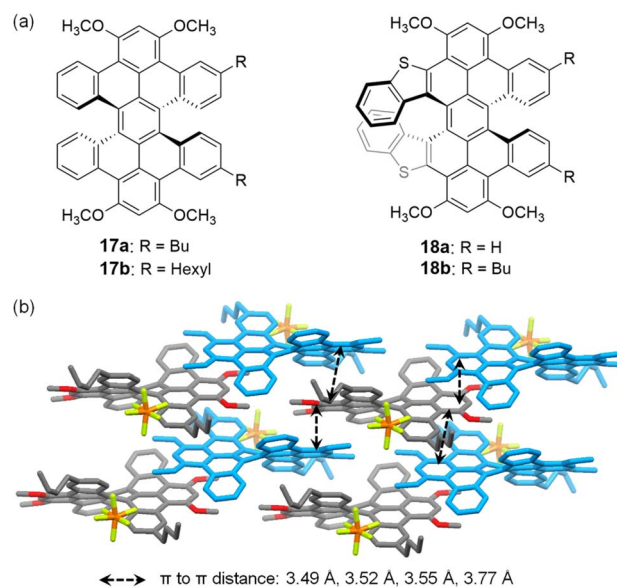
Fig. 6 (a) Double helicenes 17a/b and 18a/b ; (b) \pi - \pi stacking in the crystal of 17a^{\bullet+}\text{PF}_6^- , where the (M, M) enantiomer is shown in blue, and the (P, P) enantiomer is colored according to the elements. Reproduced with permission from ref. 40. Copyright 2022 American Chemical Society.
