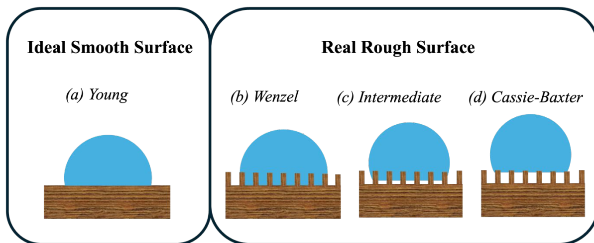
Figure 5. Schematic depiction of the surface roughness effect on the solid surface wetting by a droplet on a) an ideal smooth surface, b) Wenzel state, c) intermediate state between Wenzel and
