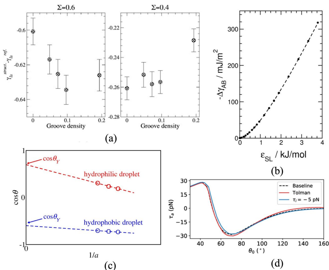
Figure 9. (a) Solid-liquid surface free energy difference as a function of the groove number density per unit area in rough surface systems (in reduced units). Reproduced with permission from reference. 159 Copyright (2010) AIP Publishing. (b) Variations of -\Delta\gamma_{AB} (equivalent to W_{ad} ) over the range of \epsilon_{SL} values considered in the study of Leroy and Müller-Plathe 160 using the “dry-surface” method. The dashed lines are guides to the eye. Reproduced with permission from reference. 160 Copyright (2015) American Chemical Society. (c) Schematic illustrating linear fits (dashed lines) to \cos\theta versus 1/a . \theta is the contact angle and a is the radius of the 3-phase contact line. Reproduced with permission from reference; 161 Copyright 2019 Elsevier. (d) The apparent line tension, \tau_a , versus the Young contact angle \theta_0 . The curve shows an asymmetric U-shaped trend and a sign change at intermediate wettability, illustrating that the extracted \tau_a depends strongly on wetting state. The dashed line is the baseline prediction, while the red and blue curves show the small changes obtained when a Tolman correction and an assumed intrinsic line tension are included. Reproduced with permission from reference. 162 Copyright 2023 American Physical Society.
