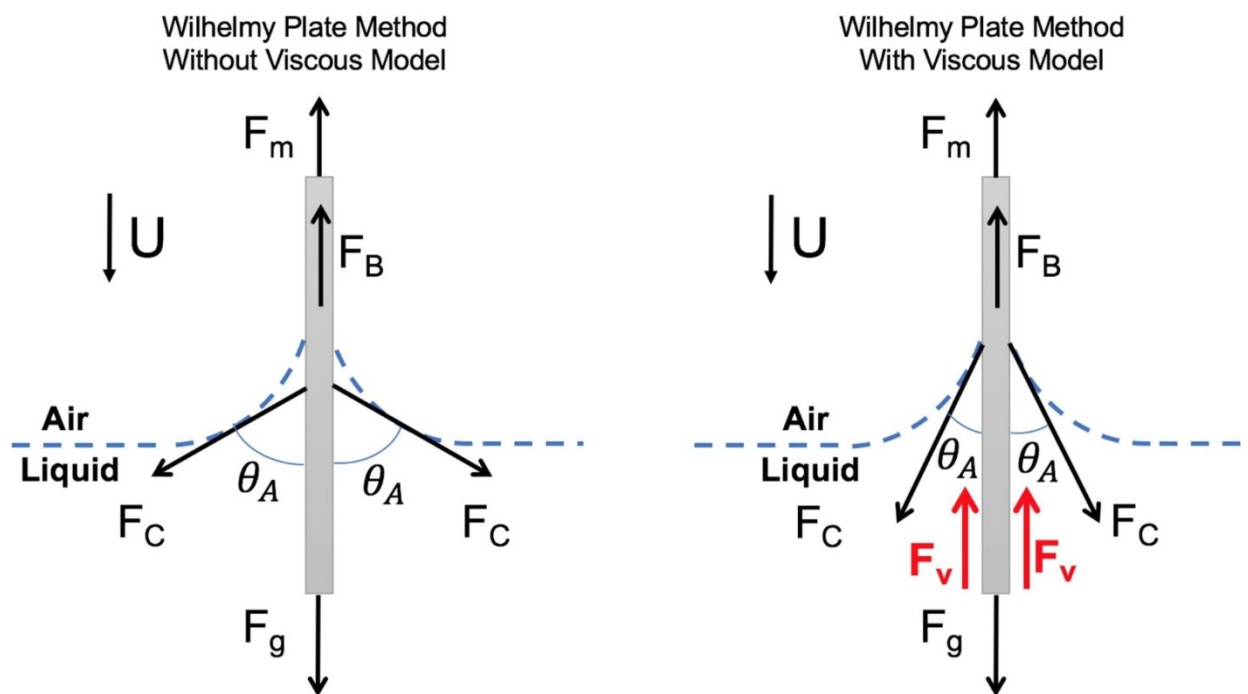
Figure 6. Effect of viscous force on dynamic contact angle measurement using the Wilhelmy plate method. Reproduced with permission from reference 98 . Copyright 2018 Elsevier.
