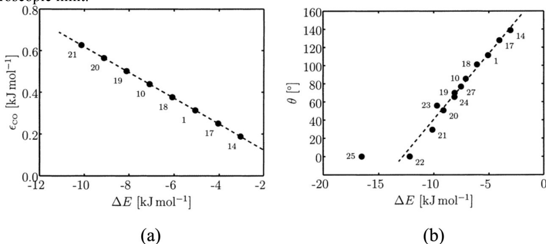
Figure 8: (a) Relation between different Lennard-Jones parameters \epsilon_{CO} considered in the study of Werder et al. 39 and the water monomer binding energy \Delta E on graphite. The numbers 14–21 denote different sets of interaction parameters considered by the authors. The dashed line is a linear fit to the data points. (b) Contact angle \theta of water droplets on graphite as a function of the binding energy \Delta E of a single water molecule obtained from different Lennard-Jones parameters considered by Werder et al. 39 . The dashed line is a linear fit excluding the cases 22, 25, and 27. Reproduced with permission from reference. 39 Copyright (2003) American Chemical Society.
