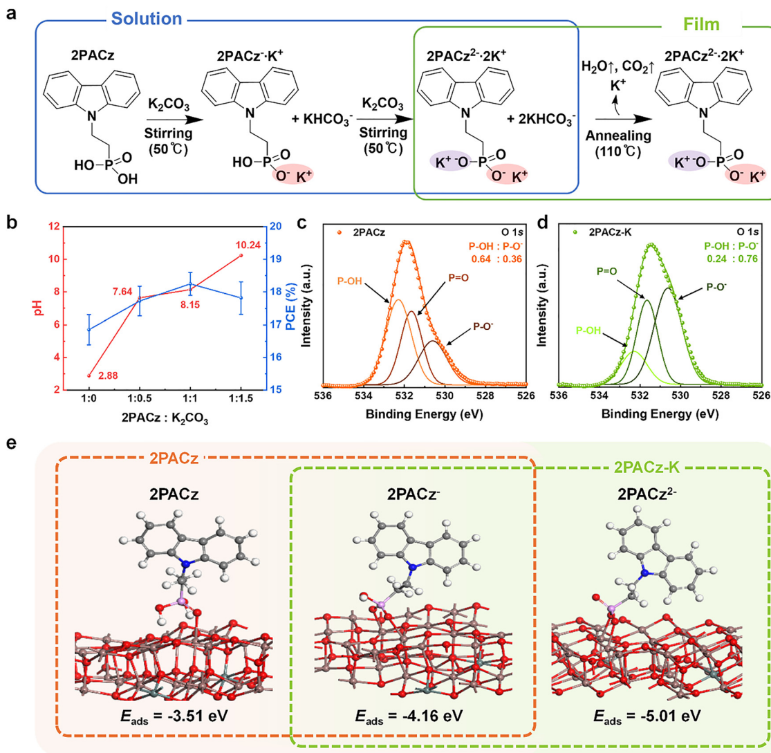
Fig. 1 (a) Schematic illustration of stepwise deprotonation of 2PACz mixing with \text{K}_2\text{CO}_3 (1 : 1 molar ratio). (b) pH values of mixed 2PACz : \text{K}_2\text{CO}_3 solutions and the corresponding PCEs of WBG PSCs. (c) and (d) O 1s XPS spectra of 2PACz and 2PACz-K on glass substrates. (e) DFT-calculated adsorption energy ( E_{\text{ads}} ) of fully protonated 2PACz , mono-deprotonated 2PACz ( 2\text{PACz}^- ), and di-deprotonated 2PACz ( 2\text{PACz}^{2-} ) on the ITO surface.
