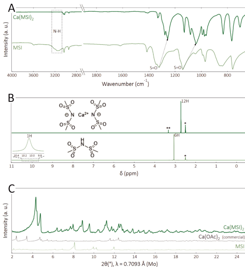
Fig. 1 (A) Infrared spectra of \text{Ca}(\text{MSI})_2 and MSI, (B) NMR spectra of MSI (* \text{DMSO-d}_6 , **water), (C) The PXRD spectra of \text{Ca}(\text{MSI})_2 , \text{Ca}(\text{OAc})_2 , and MSI.
