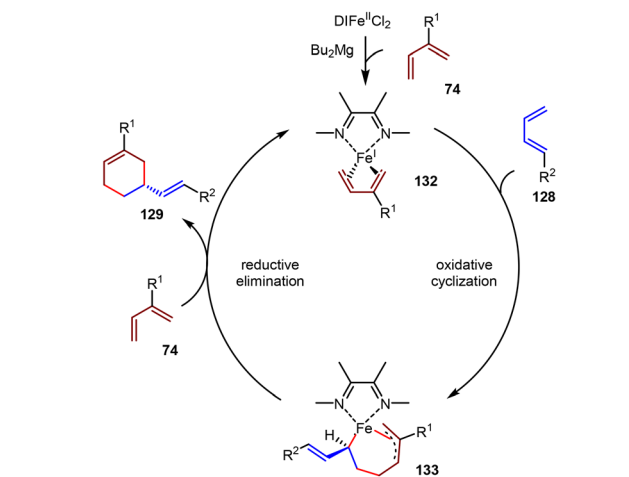
Scheme 29 Fe(I)/ \alpha -diimine-catalyzed asymmetric cross-[4+2] cycloadditions of unactivated 1,3-dienes.
