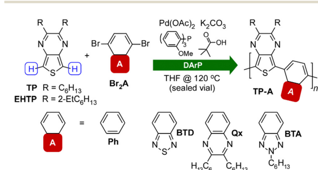
Scheme 1 Synthesis of thieno[3,4- b ]pyrazine-acceptor frameworks.
