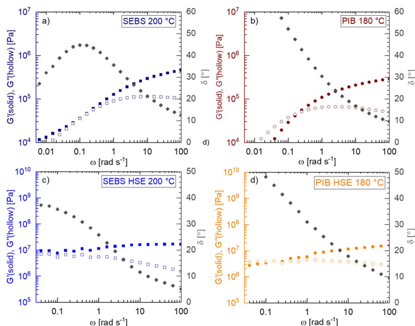
Fig. 9 G' and G'' moduli (left axis) and \delta (right axis) as a function of angular frequency for (a) SEBS at 200^\circ\text{C} , (b) PIB at 180^\circ\text{C} , (c) SEBS HSE at 200^\circ\text{C} and (d) PIB HSE at 180^\circ\text{C} .
