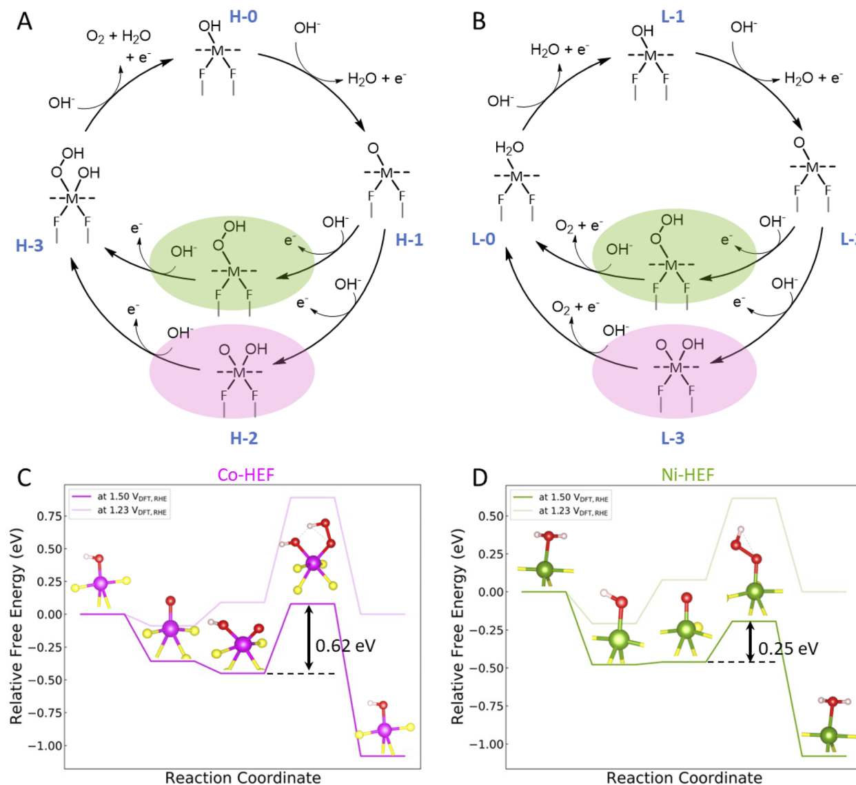
Fig. 5 Reaction-mechanism of OER on HEF-surface: (A and B) proposed adsorbate evolution mechanism for Co (pink) and Ni (green) involving the formation of ^*OOH species as a rate-determining step via ^*O-O coupling from ^*Ni-O and ^*Co-(O)(OH) species. "H" and "L" represent suggested oxidation states for metal ions that could be accessible in higher and lower potential regimes ( V_{RHE} ) to derive the kinetics of reactions. (C and D) Free energy diagrams for possible OER active metals (Co and Ni) under consideration, at thermodynamic potential ( 1.23 V_{RHE} ) and the potential considered for the calculation of experimental Tafel slope ( \approx 1.50 V_{RHE} ).
