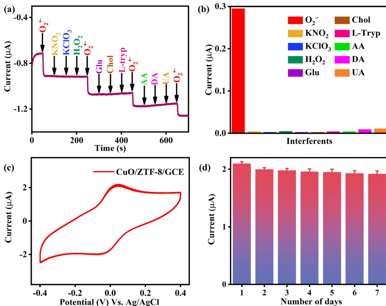
Fig. 6 (a) Effect of interfering species on the amperometric ( i – t ) current response of the CuO/ZTF-8/GCE for 25 \mu\text{M} \text{O}_2^{\cdot-} in 0.1 M phosphate buffer (pH 7; \text{N}_2 saturated). (b) Corresponding columnar current response. (c) Cyclic voltammogram of CuO/ZTF-8/GCE at a scan rate of 50 \text{mV s}^{-1} in 0.1 M phosphate buffer (pH 7, \text{N}_2 saturated) for 100 continuous cycles. (d) Columnar diagram of the current response obtained for CuO/ZTF-8/GCE from CV studies for seven consecutive days.
