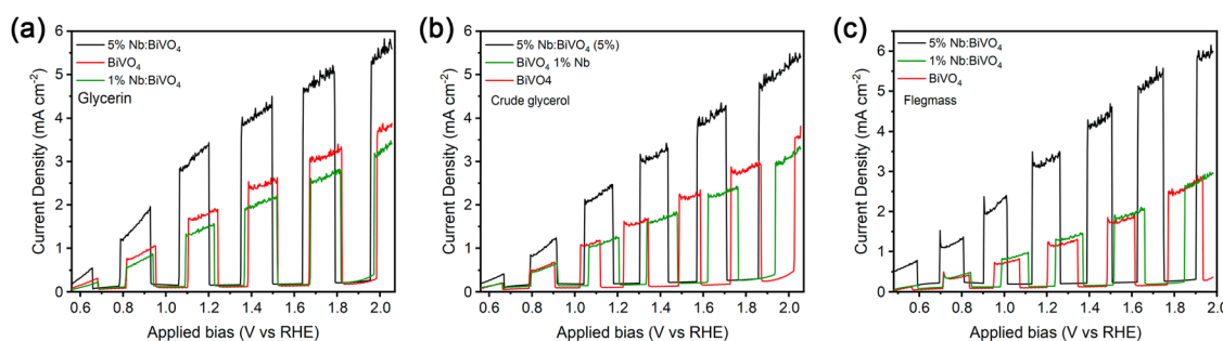
Fig. 7 Light-chopped linear sweep voltammograms of pristine BiVO 4 , 1% and 5% Nb : BiVO 4 films in (a) glycerin 10% v/v in K 2 SO 4 0.1 M, (b) crude glycerol 10% v/v in K 2 SO 4 0.1 M and (c) raw flegmass with added 0.1 M K 2 SO 4 .
