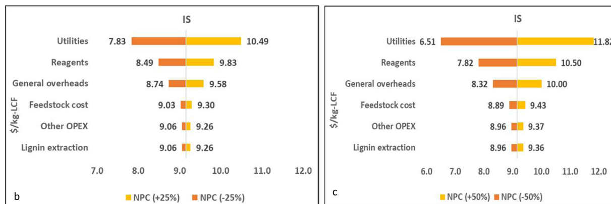
Fig. 7 Cost analysis (base case) for carbon fibre production via redissolution (RS) and integrated spinning (IS). (a) Production cost of lignin carbon fibre. (b) and (c) Sensitivity analysis on utility cost (mainly energy), overheads, raw materials, utility cost and feedstock cost for the integrated fibre spinning process.
