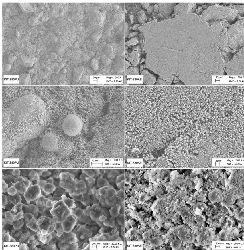
Fig. 2 SEM images of the calcined KIT-Z80PU (left) and KIT-Z80AE (right) catalyst.
