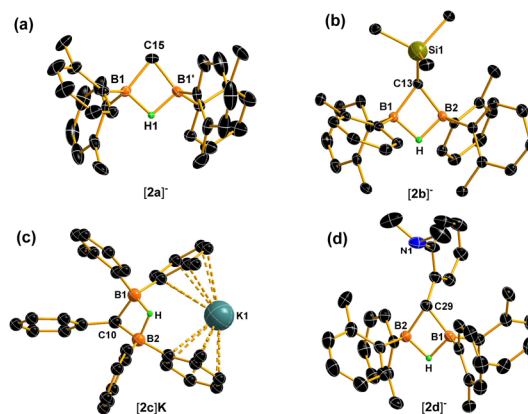
Fig. 1 Molecular structures of [2a] – , [2b] – , [2c]K and [2d] – (all hydrogen atoms and cations are omitted for clarity except for the bridging H atoms). Selected atom...atom distance (Å) and bond angles (deg.), (a) [2a]Li: B1...B1' = 1.982(5); B1–C15–B1' = 76.1(2). (b) [2b]Li: B1...B2 = 1.9578(18); B1–C13–B2 = 74.04(8). (c) [2c]K: B1...B2 = 1.971(2); B1–C10–B2 = 75.03(10). (d) [2d]Li: B1...B2 = 1.963(3); B1–C29–B2 = 73.94(12).
