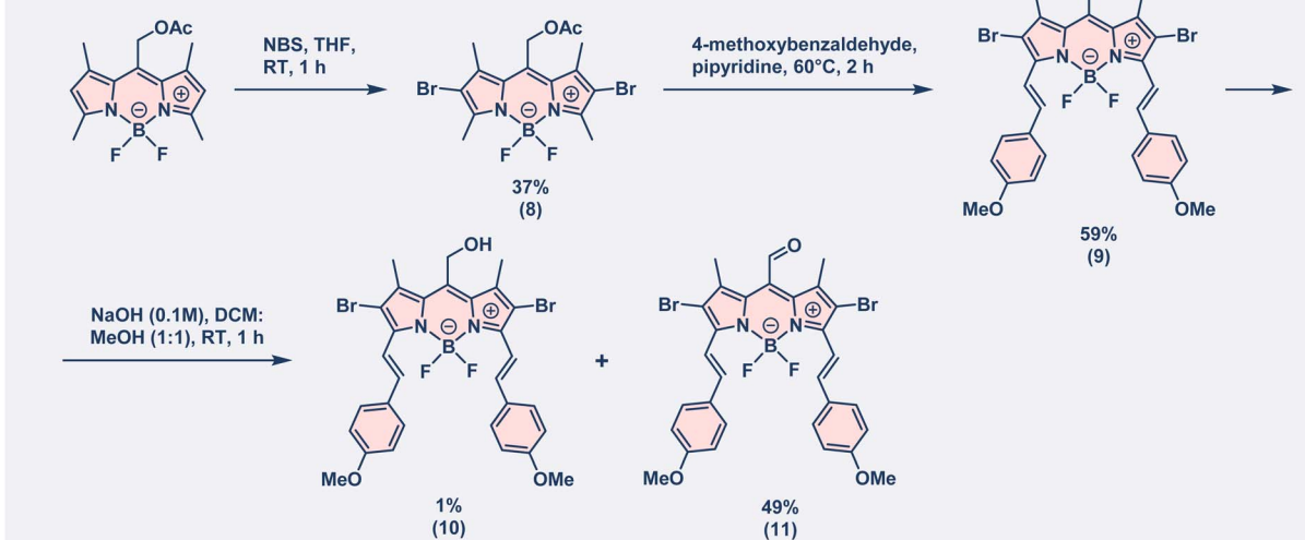
Scheme 1 The synthetic scheme above illustrates the pathways used to synthesize BODIPY derivatives described in this study.
