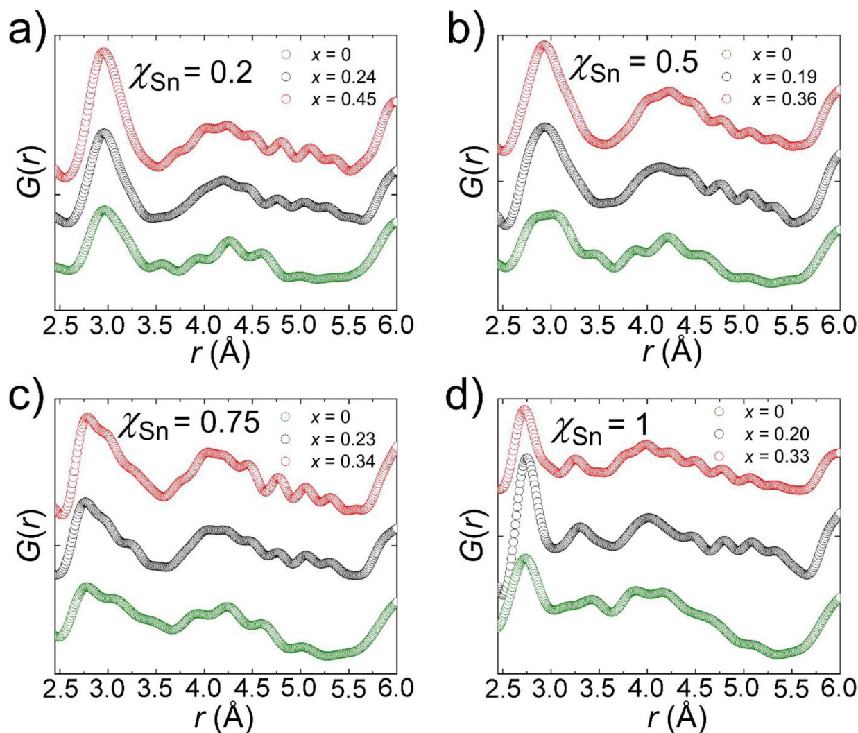
Fig. 7 Experimental pair distribution function (PDF) curves for representative compounds in the \text{FA}_{1-x}\text{Sn}_x\text{Pb}_{1-y}\text{Sn}_y\text{Br}_3 family of perovskites in four panels (a–d) depending on the experimentally determined Sn fraction ( \chi_{\text{Sn}} ) and ethylenediammonium fraction ( x ). Here the PDF of \text{FASnBr}_3 is plotted from our previous works for comparison. 51
