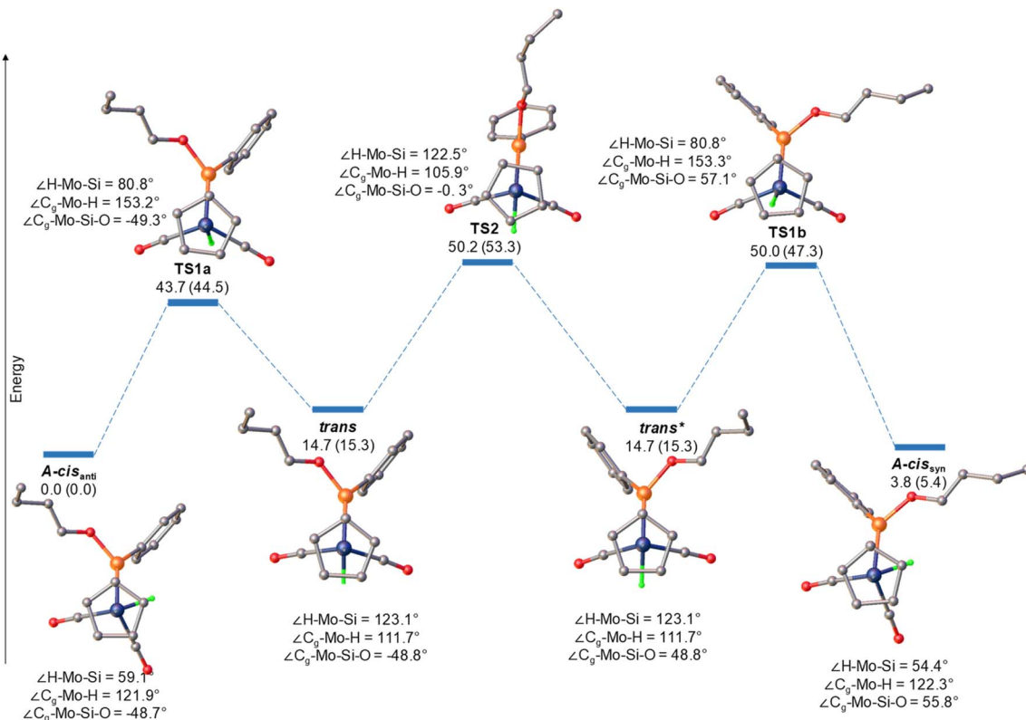
Fig. 13 Reaction profile for the diastereomerization of A- cis anti to A- cis syn ; Olex plots of the calculated structures of A- cis anti , A- cis syn , the transition states (TS1a, TS2 and TS1b) and the intermediates trans and trans * (top views) with their relative zero-point vibrational energy corrected inner energies \Delta U(0\text{ K}) (kJ mol -1 ) and standard free energies \Delta G^\circ (kJ mol -1 ) (values in parentheses).
