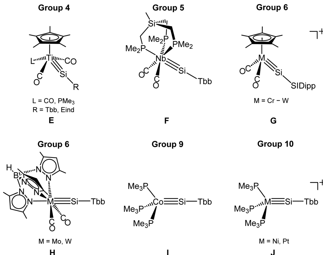
Fig. 2 Silyldyne complexes of various transition metal groups isolated and fully characterized in our group; SIDipp = C[N(Dipp)CH 2 ] 2 , Dipp = 2,6-diisopropylphenyl; Tbb = C 6 H 2 -2,6-(CH(SiMe 3 ) 2 ) 2 -4-tBu; Eind = 1,1,3,3,5,5,7,7-Et 8 -s-hydrindacene-4-yl.
