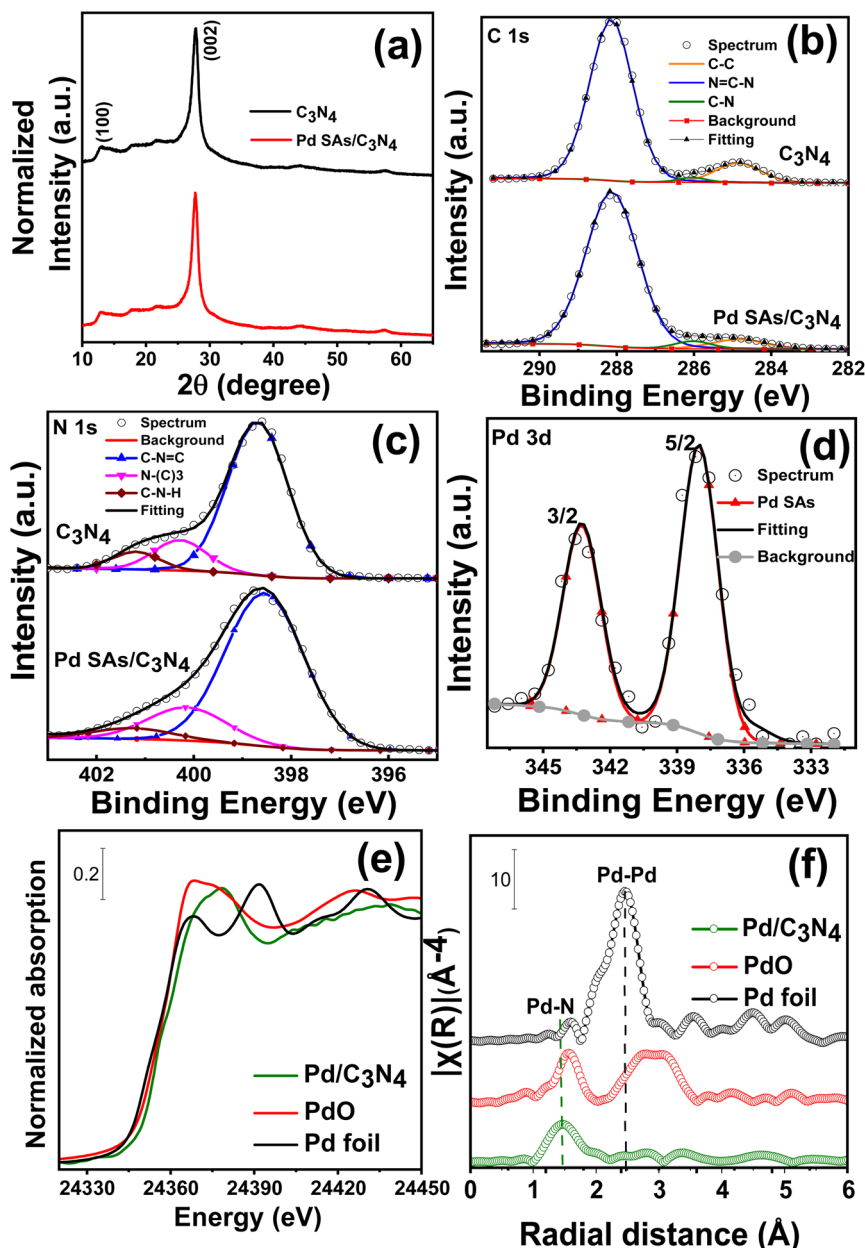
Fig. 2 (a) X-ray diffraction pattern, (b–d) XPS spectra of (b) C 1s, (c) N 1s and (d) Pd 3d for C_3N_4 and Pd\ SAs/C_3N_4 , (e) XANES spectra of Pd/C_3N_4 at Pd K-edge, and (f) Fourier transform extended X-ray absorption fine structure (FT-EXAFS) spectra of Pd\ SAs/C_3N_4 .
