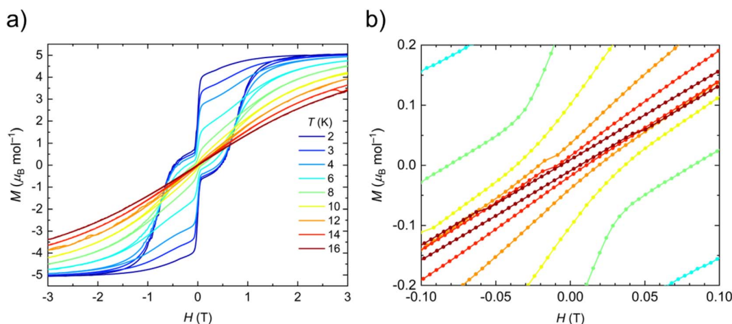
Fig. 3 (a) Hysteresis loops of 1-Dy from 2 to 16 K and -3 \text{ T} to +3 \text{ T} , sweep rate is 22 \text{ Oe s}^{-1} . (b) Hysteresis loops of 1-Dy at 6–16 K between -0.1 and +0.1 \text{ T} , sweep rate is 22 \text{ Oe s}^{-1} . Hysteresis is considered open until T_{\text{H}} = 14 \text{ K} .
